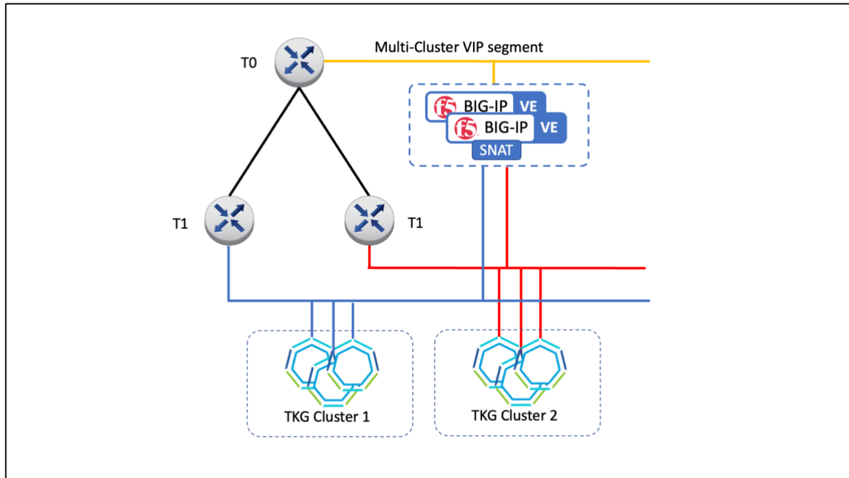
Figure 131 - A BIG-IP cluster for multiple TKG workload clusters.
