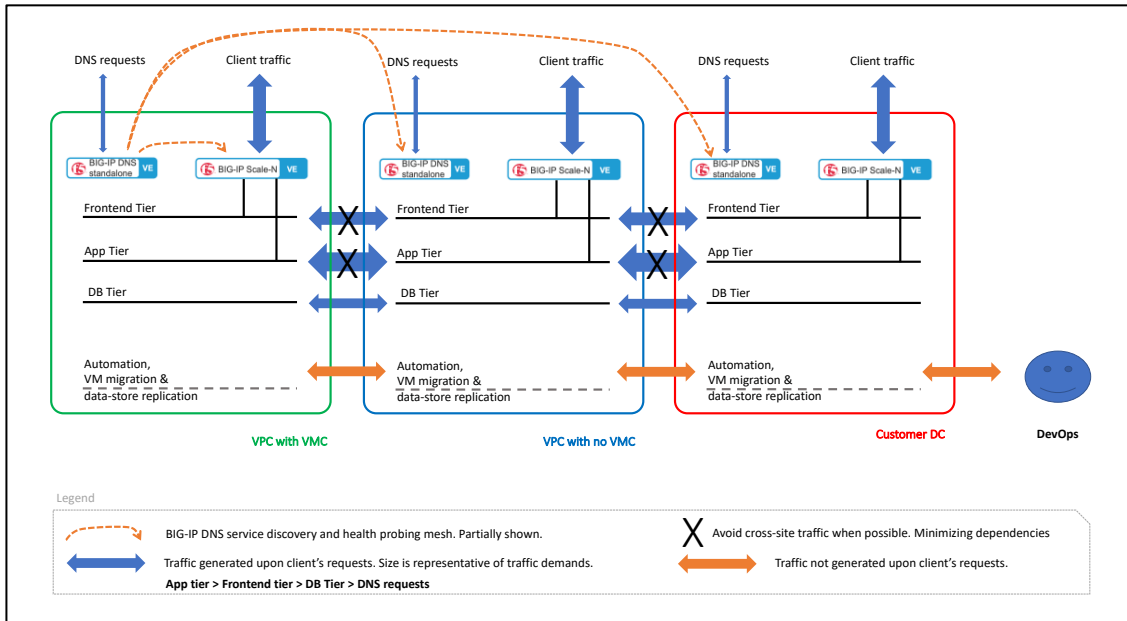
Figure 119 - Typical multi-cloud arrangement with most relevant traffic patterns.
