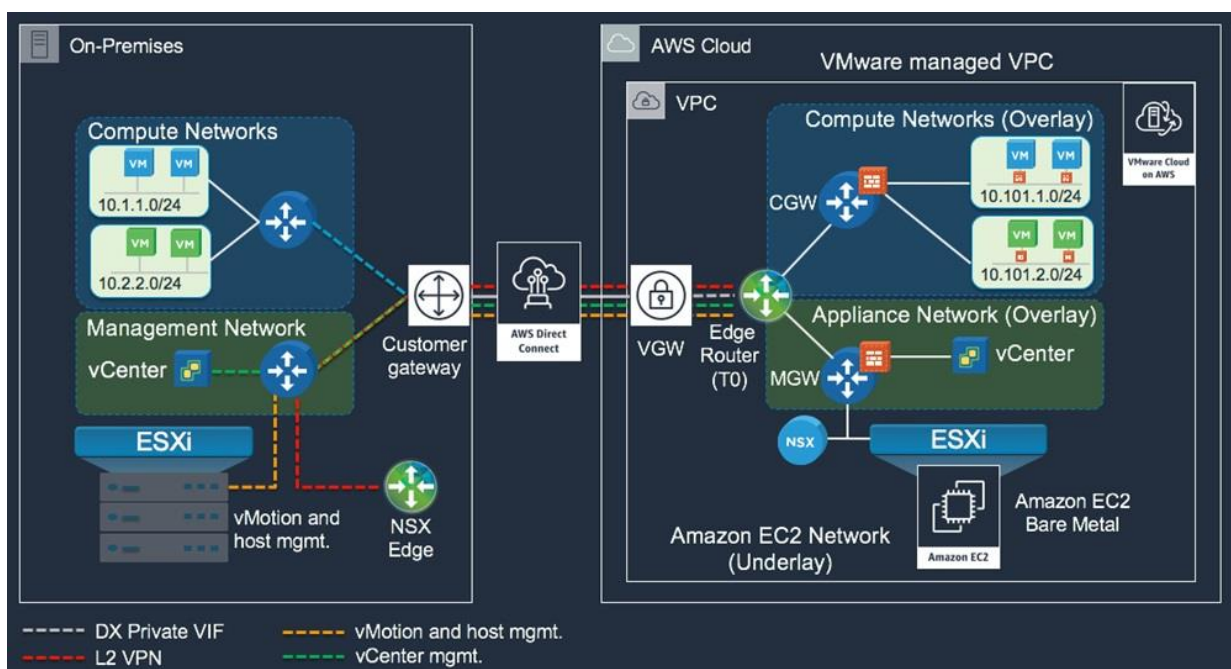
Figure 107 - Sample architecture showing some connectivity options
