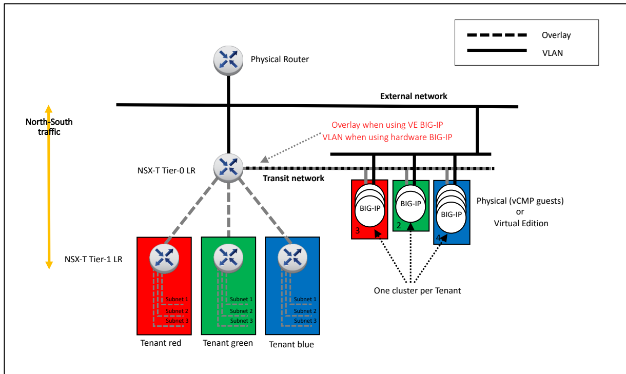
Figure 96 – Topology C with multiple tenants shown.
