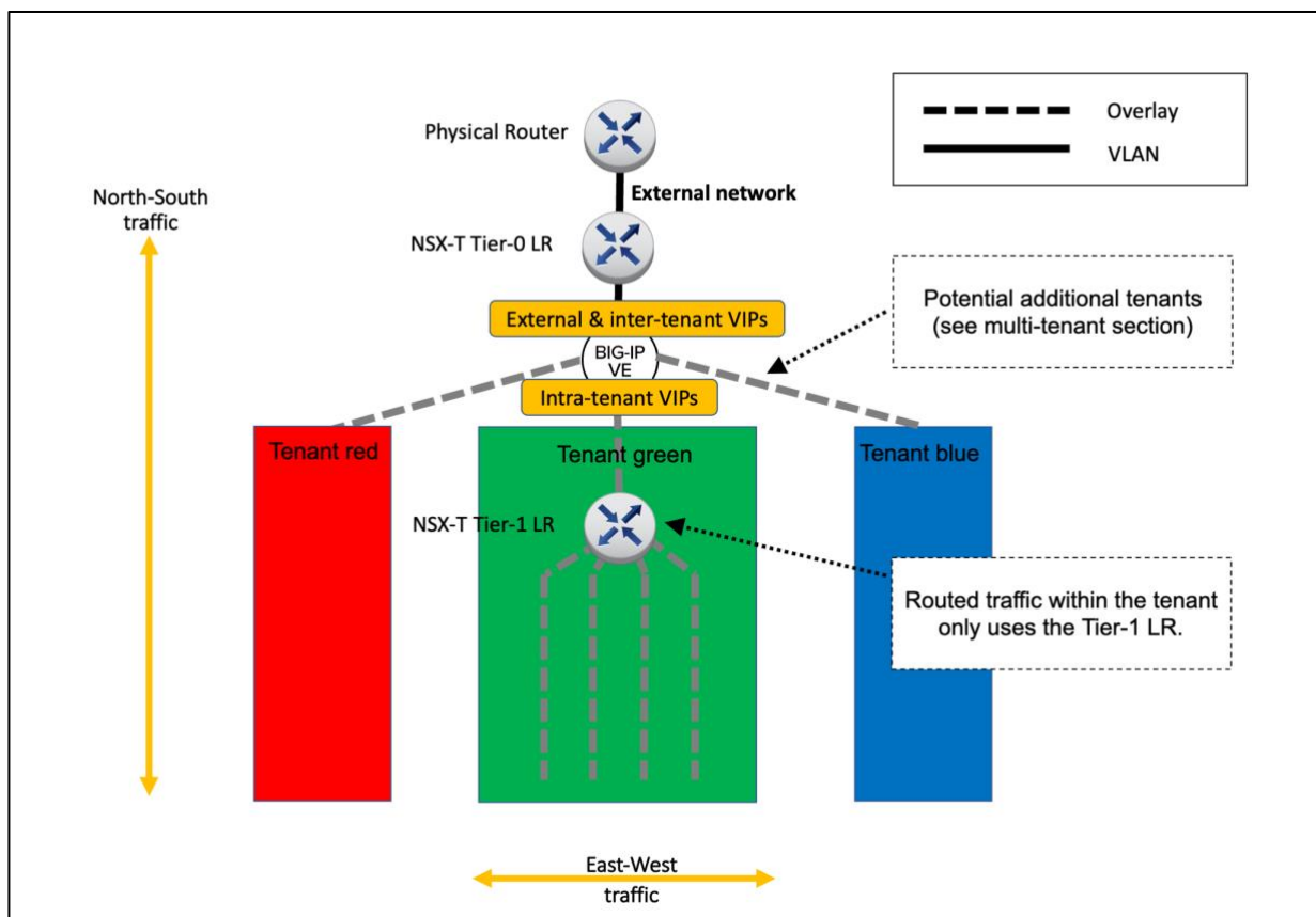
Figure 63 – Overview of BIG-IPs inline-connected to an NSX-T's Tier-1 Gateway.
