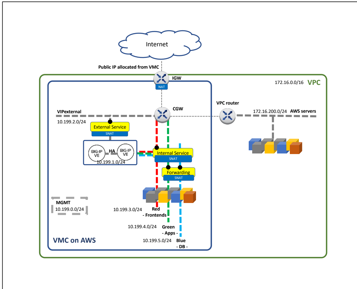
Figure 108 - Sample Topology D for VMC
