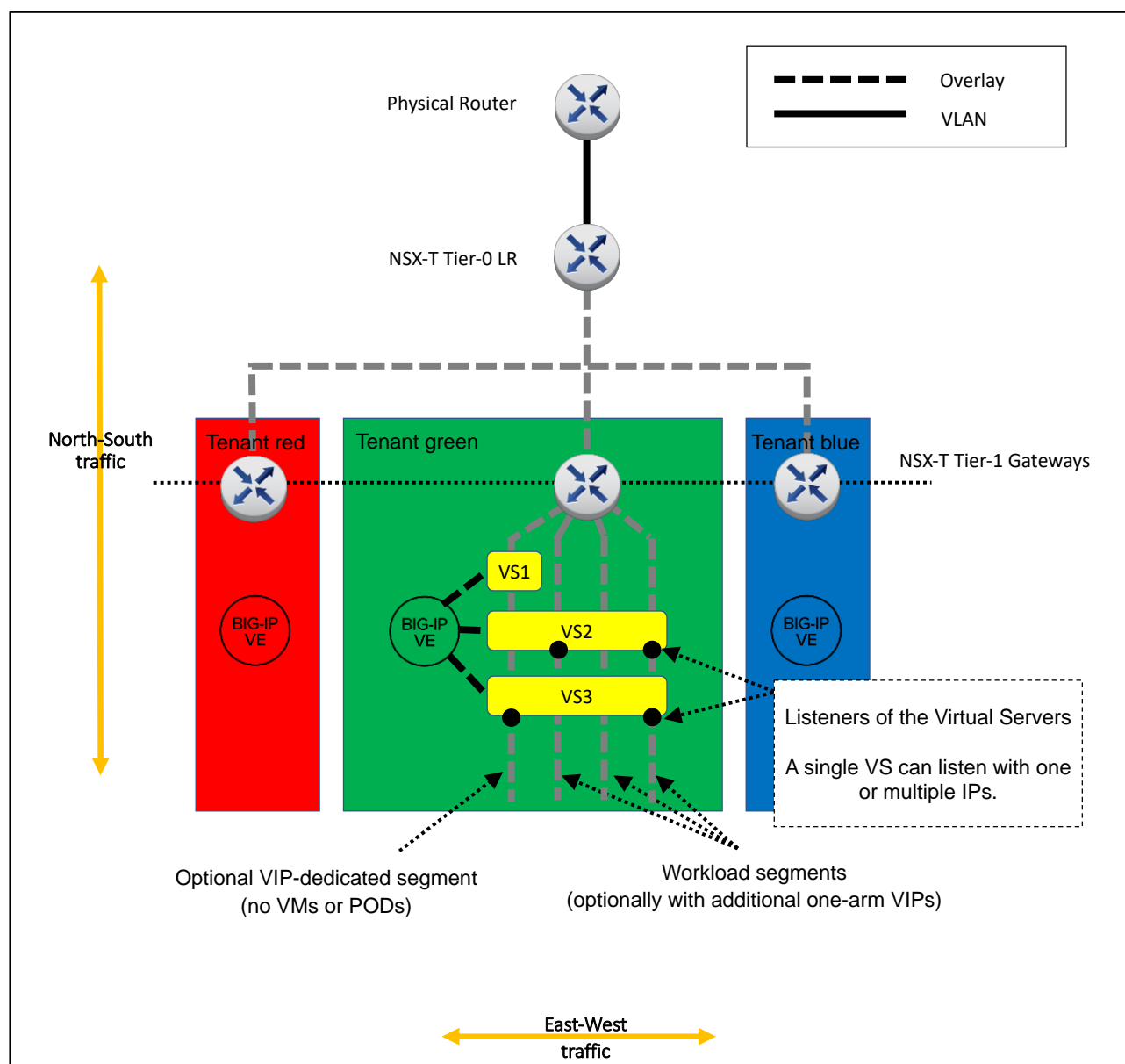
Figure 97 – Topology D overview (simplified view without HA components).
