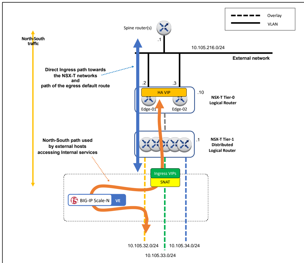
Figure 98 – Topology D example implementation – North/South traffic flows.
