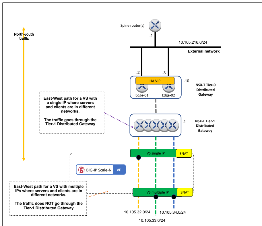
Figure 102 – Topology D implementation used through this section.
