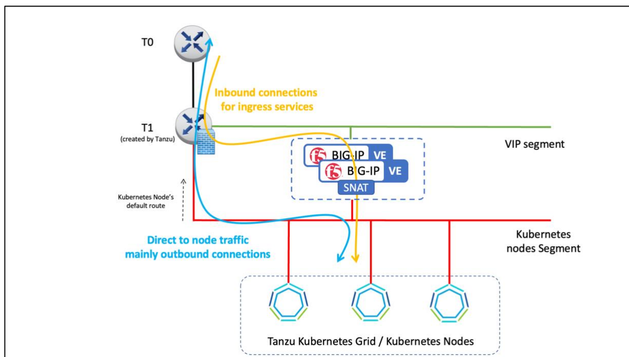
Figure 130 - A BIG-IP cluster per TKG workload cluster.
