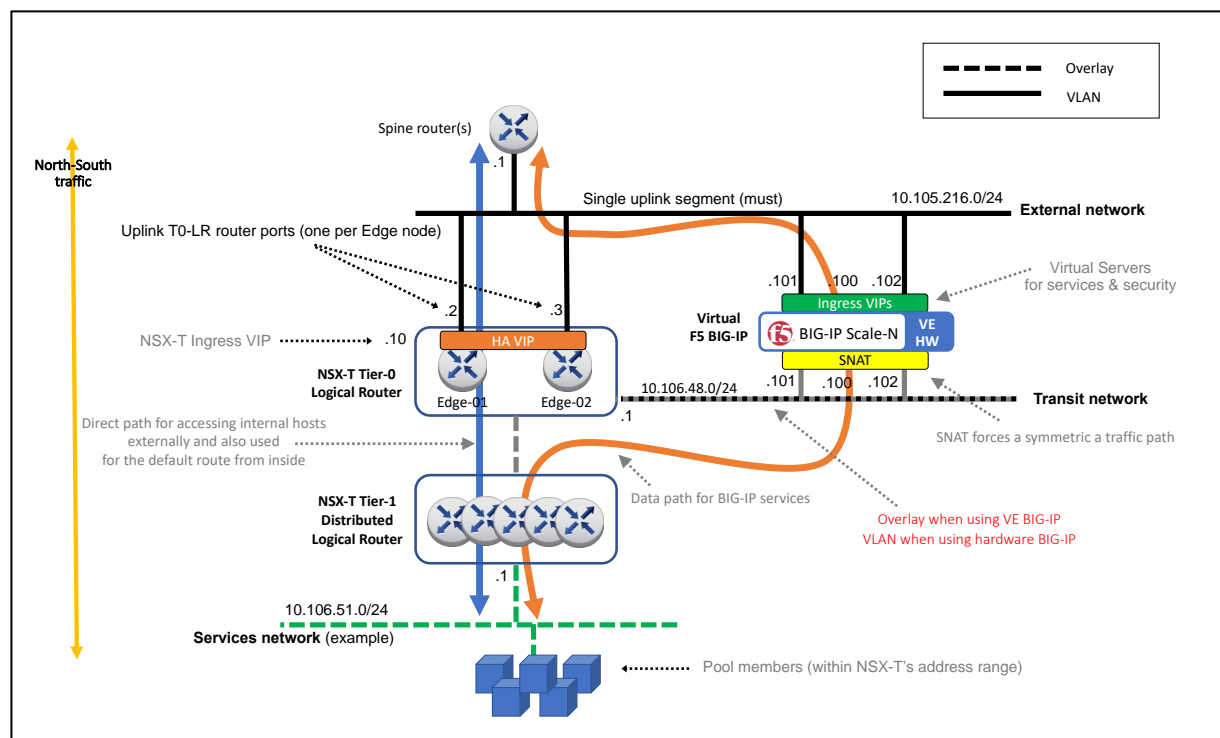
Figure 82 – Topology C example implementation.
