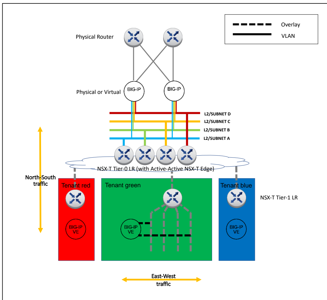
Figure 101 – Combined Topology A and D.
