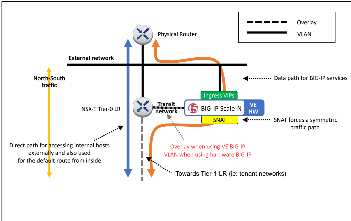
Figure 81 – Topology C overview.
