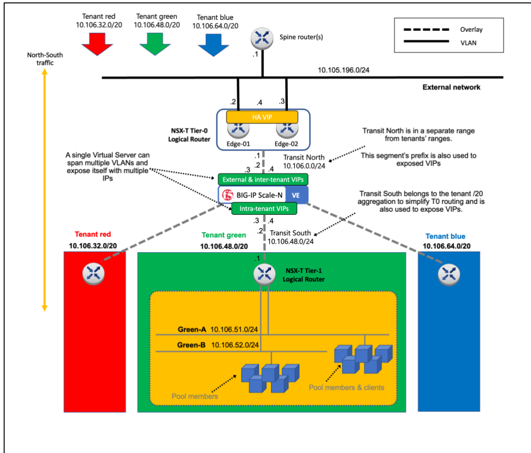
Figure 64 – Topology B extended, example implementation.
