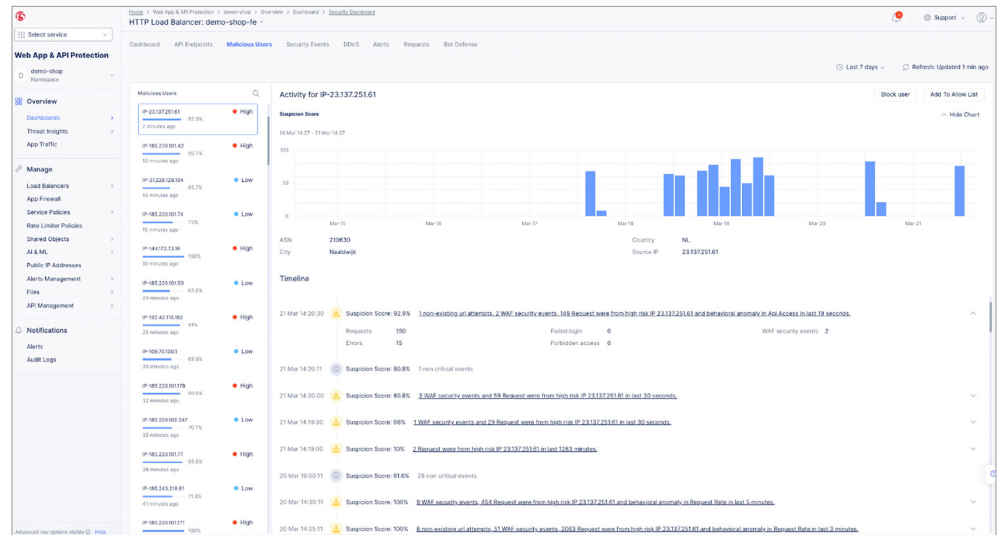
Figure 5: Malicious User functionality—correlates WAF events, abnormal API access behavior, failed login attempts, and so forth, for app and API endpoints, flagging these for operations teams with the ability to quickly take action including block/allow list, rate limit, and more.
