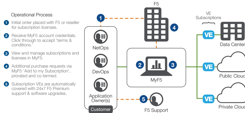
Figure 1: F5 Subscription Program makes it easy for organizations to deploy BIG-IP VEs across hybrid environments.
